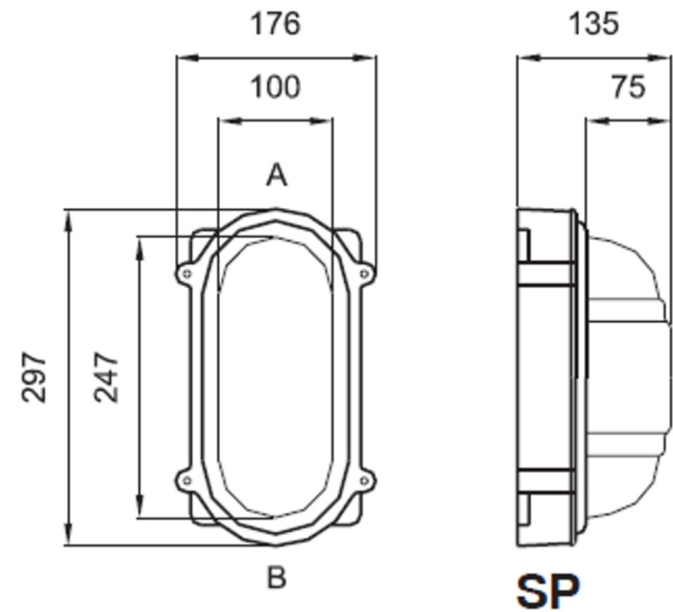
Dimensions (mm)
