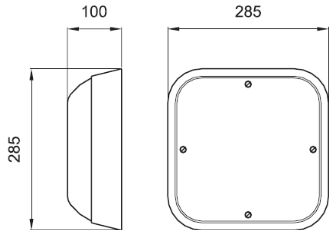
Dimensions (mm)
